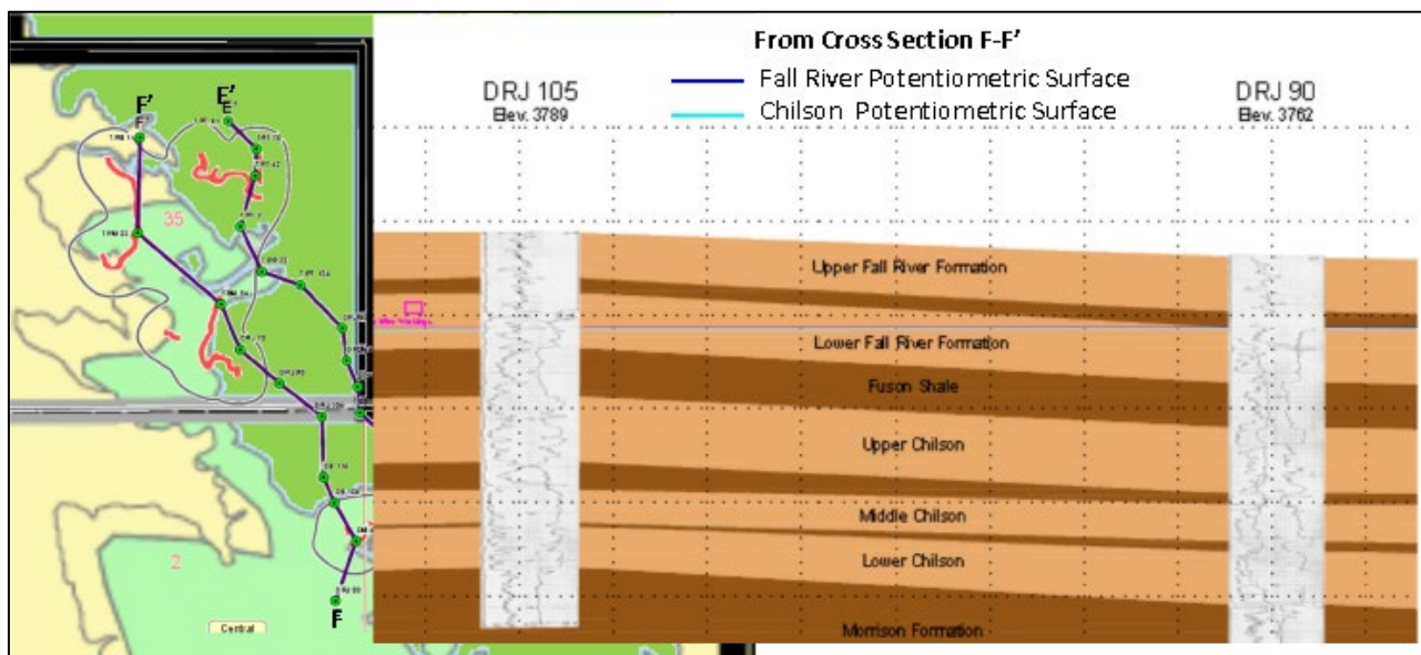
Figure 24. A Portion of Class III Permit Application Cross Section F-F' between Burdock Wellfields 7 and 8 at the Fall River Outcrop Area.
