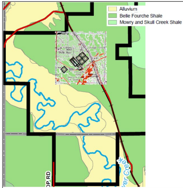
Figure 8b. Dewey Area Pond Locations for the Land Application Disposal Method and the Surface Geology (Source: Class III Permit Application Figure 6.3)
