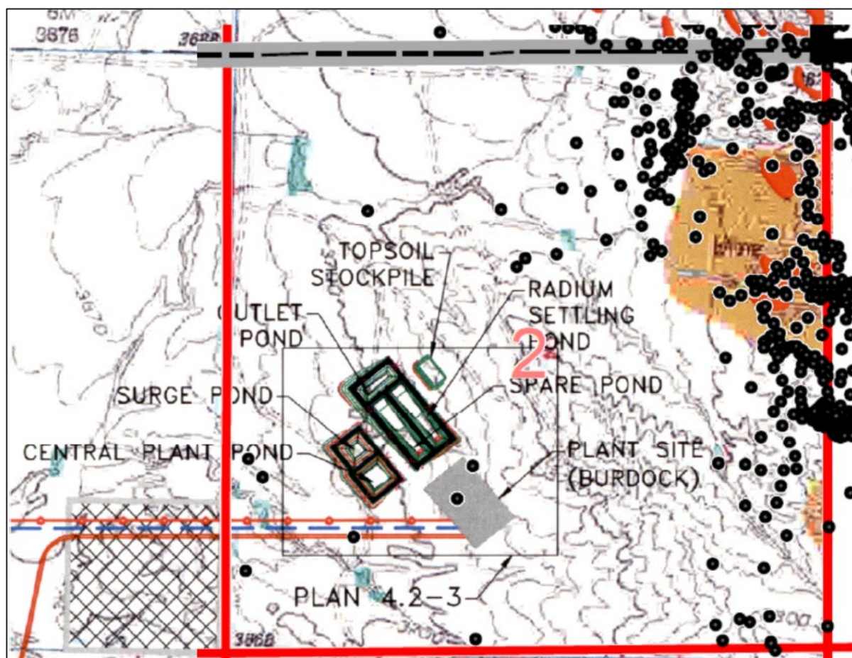
Figure 14a. Burdock Area Pond Locations for the Deep Injection Well Disposal Method and UIC Class III Permit Application Figure 4.2 Dewey-Burdock Drillhole Map
